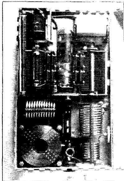
BACK VIEW OF AIRPLANE TRANSMITTER WITH COVER OPEN
