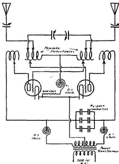
THE PUSH-PULL SERIES FEED CIRCUIT OF THE WFBT TRANSMITTER
